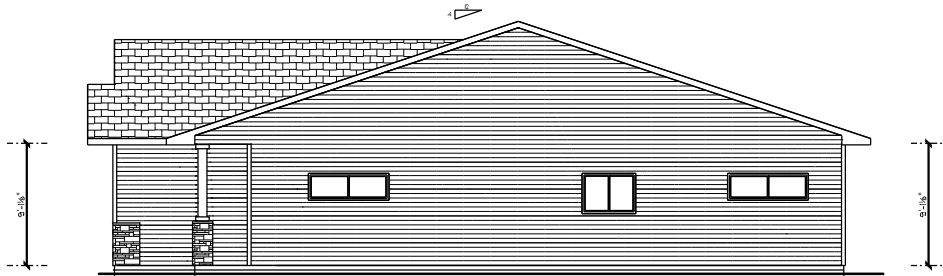
RIGHT ELEVATION 1/8" = 1'-0"
