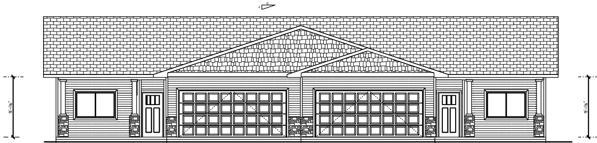
FRONT ELEVATION 1/8" = 1'-0"
