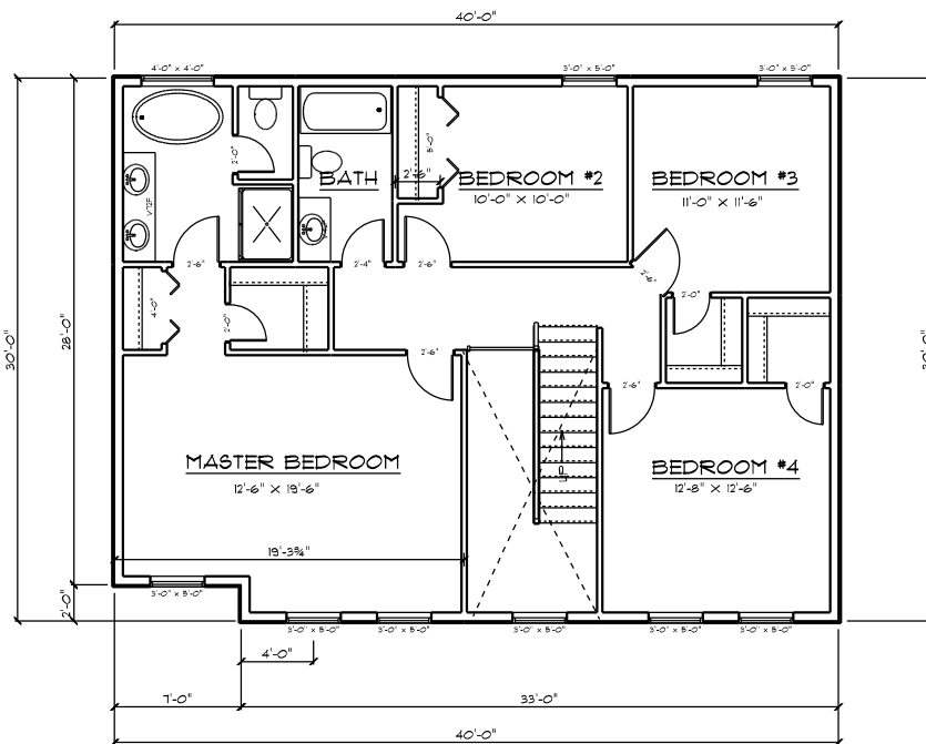
SECOND FLOOR PLAN 1186 FINISHED SQ FEET
