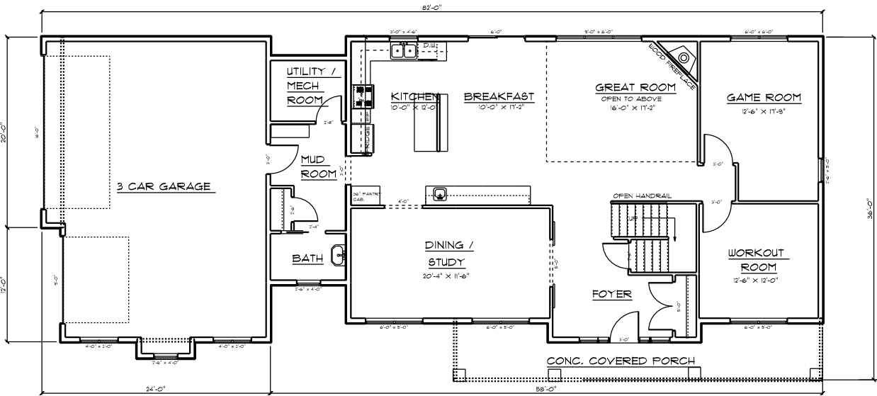
MAIN FLOOR 1761 SQ FT
